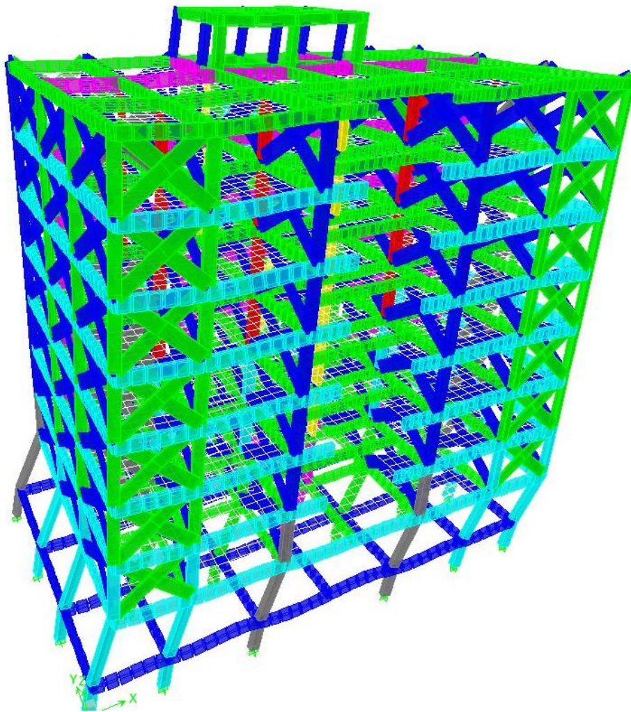
Dynamic Analysis for Soft Story (8 Storied Building at Mirpur DOHS)
