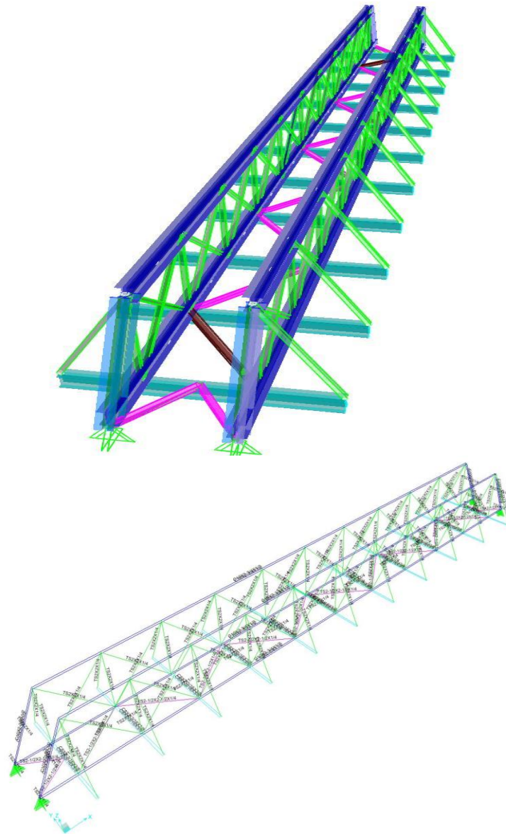
Design Fiber-reinforced Polymer Bridge
