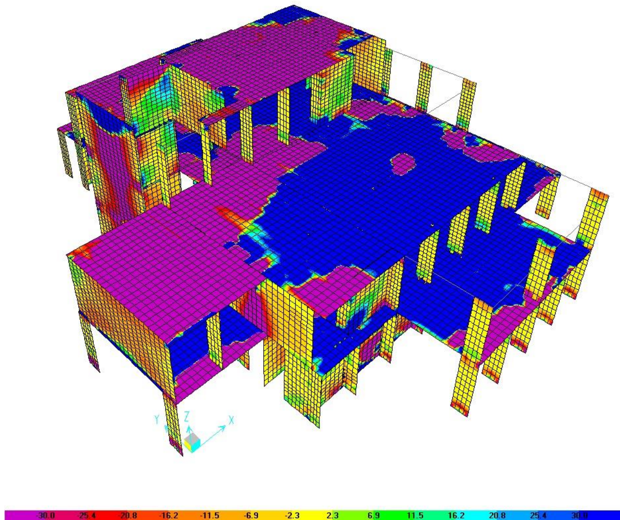
Seismic Analysis and retrofitting of Existing Structure, Client US Embassy
