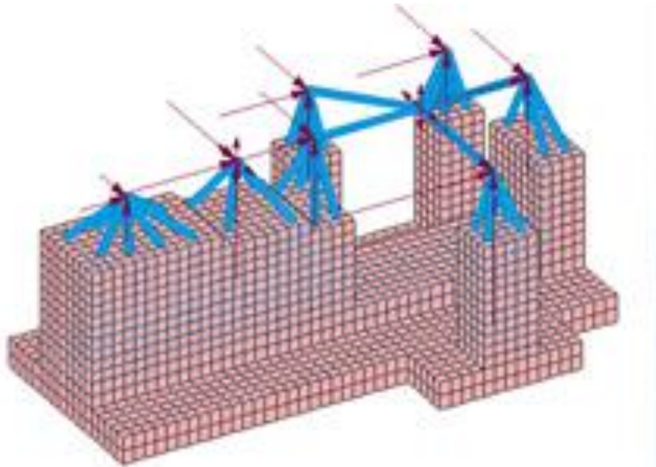
Design of Foundation for Vibratory Load
